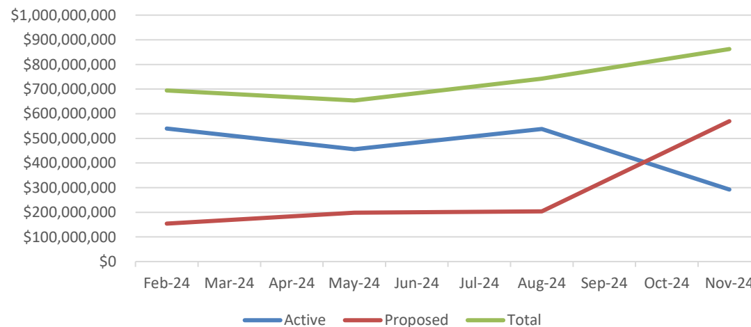
Category 1, 2, 3 Trend
